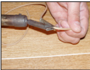
Figure 1 3.5mm welding thread in 4.0 mm tip.
